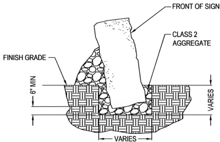
FOOTING DETAIL
